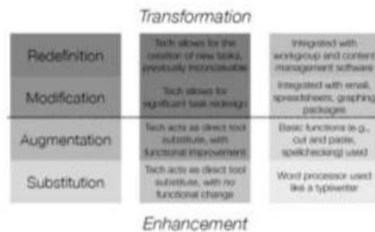
Gambar 2 Model SAMR
